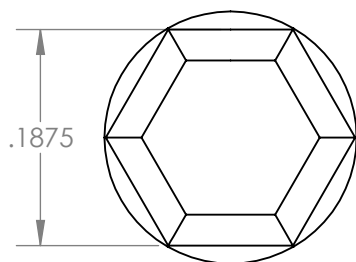
DETAIL A SCALE 6 : 1
